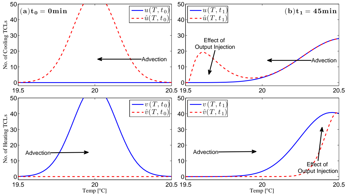
Fig. 5. The left side (a) and right side (b) depict snapshots of the true and estimated states, at times t_0 = 0 min and t_1 = 45 min, respectively. In (a), the observer is initialized with an incorrect state, namely \hat{u}(T, t_0) = v(T, t_0) and \hat{v}(T, t_0) = u(T, t_0) . Subplot (b) depicts how the output error injection corrects the “outlet” end of the flow, whereas the system’s natural advection corrects the “inlet” end.
